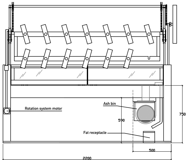
FRONT CROSS SECTION
