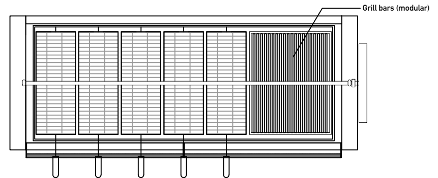
TOP VIEW (ALTERNATE SETUP)
