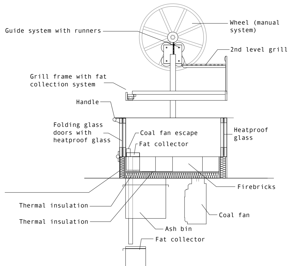
CROSS SECTION
